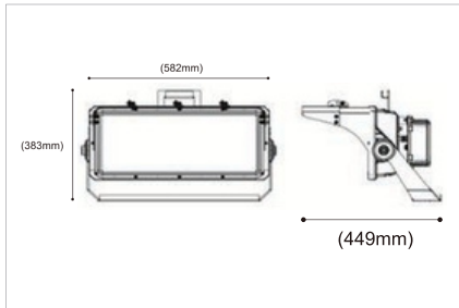
SIZE | LED-FLD084 800W
