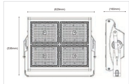
SIZE | LED-FLD063 800W
