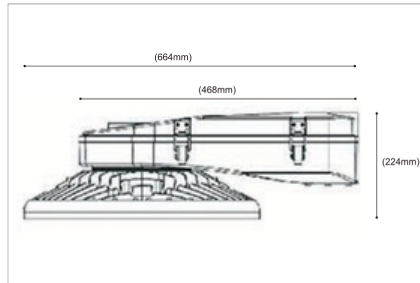
SIZE | LED-FLD072 315W
