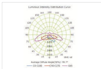
LIGHT DISTRIBUTION
