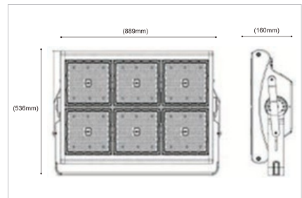
SIZE | LED-FLD066 1500W
