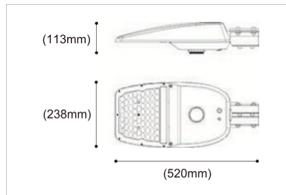
SIZE | LED-STQ-75W
