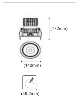
SIZE | LED-D519-30W
