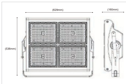
SIZE | LED-FLD064 1000W
