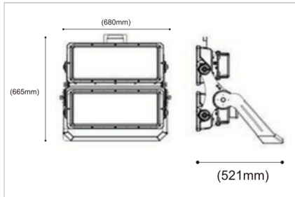
SIZE | LED-FLD087 1500W
