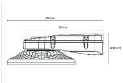
SIZE | LED-FLD074 460W
