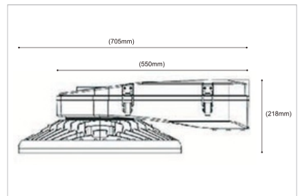
SIZE | LED-FLD076 720W
