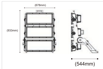
SIZE | LED-FLD088 1800W
