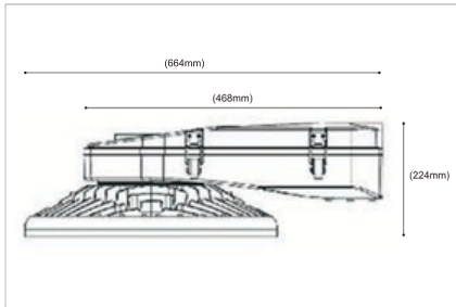
SIZE | LED-FLD071 230W
