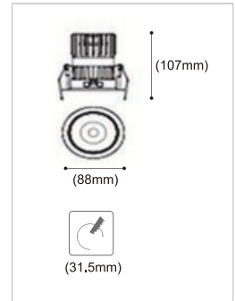
SIZE | LED-D515-10W
