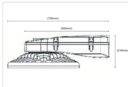
SIZE | LED-FLD075 580W
