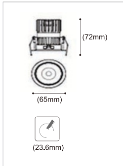
SIZE | LED-D511-7W
