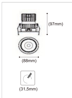
SIZE | LED-D517-10W
