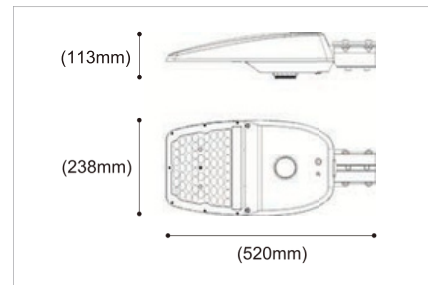
SIZE | LED-STQ-100W
