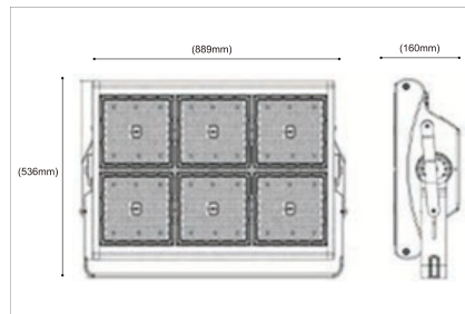
SIZE | LED-FLD065 1200W
