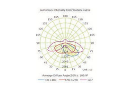
LIGHT DISTRIBUTION
