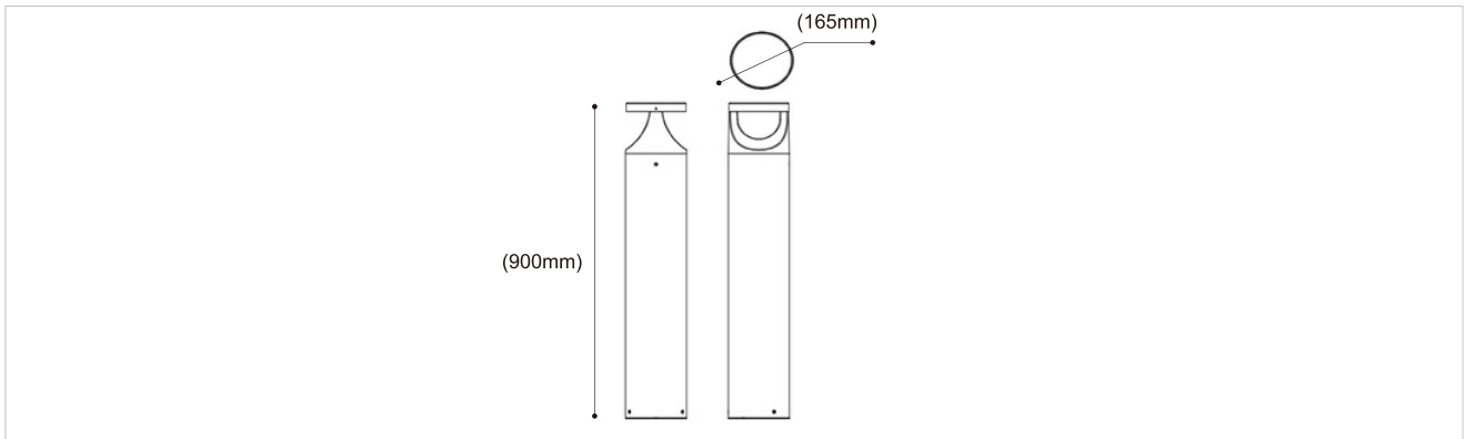
SIZE | LED-BOLED 043-24W
