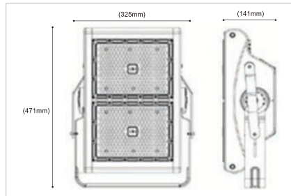
SIZE | LED-FLD062 500W
