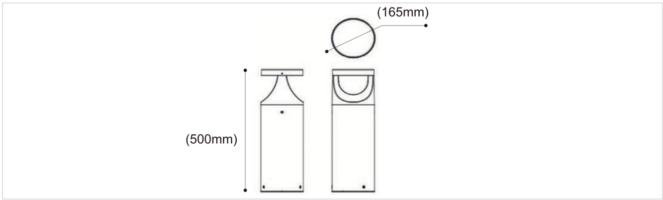
SIZE | LED-BOLED 042-14W
