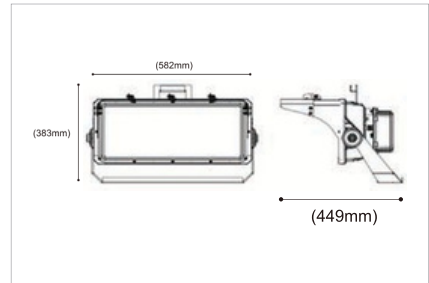
SIZE | LED-FLD086 1200W
