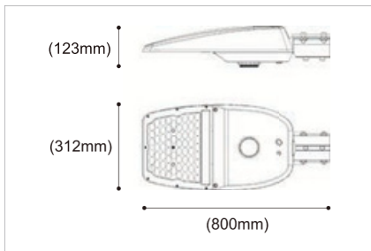
SIZE | LED-STQ-140W
