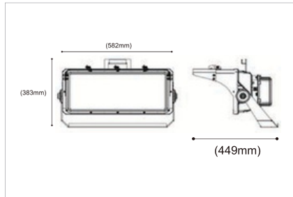
SIZE | LED-FLD085 1000W
