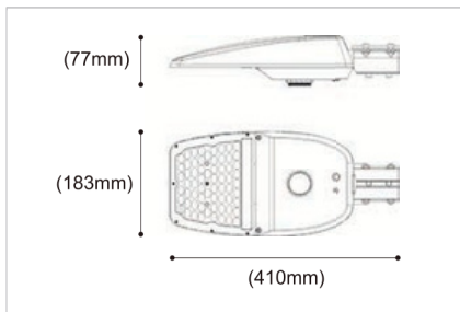
SIZE | LED-STQ-50W
