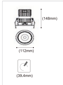
SIZE | LED-D514-25W
