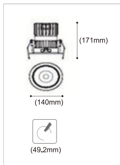
SIZE | LED-D518-30W
