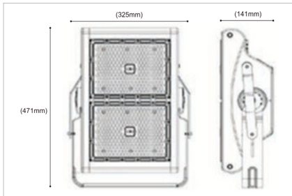
SIZE | LED-FLD061 400W
